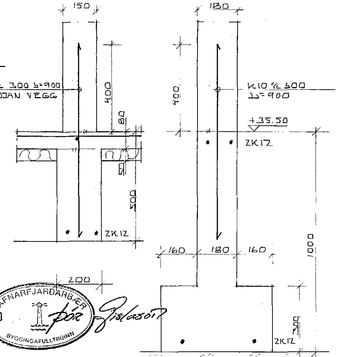
SNID H-H 1:10 SNID I-I 1:10
