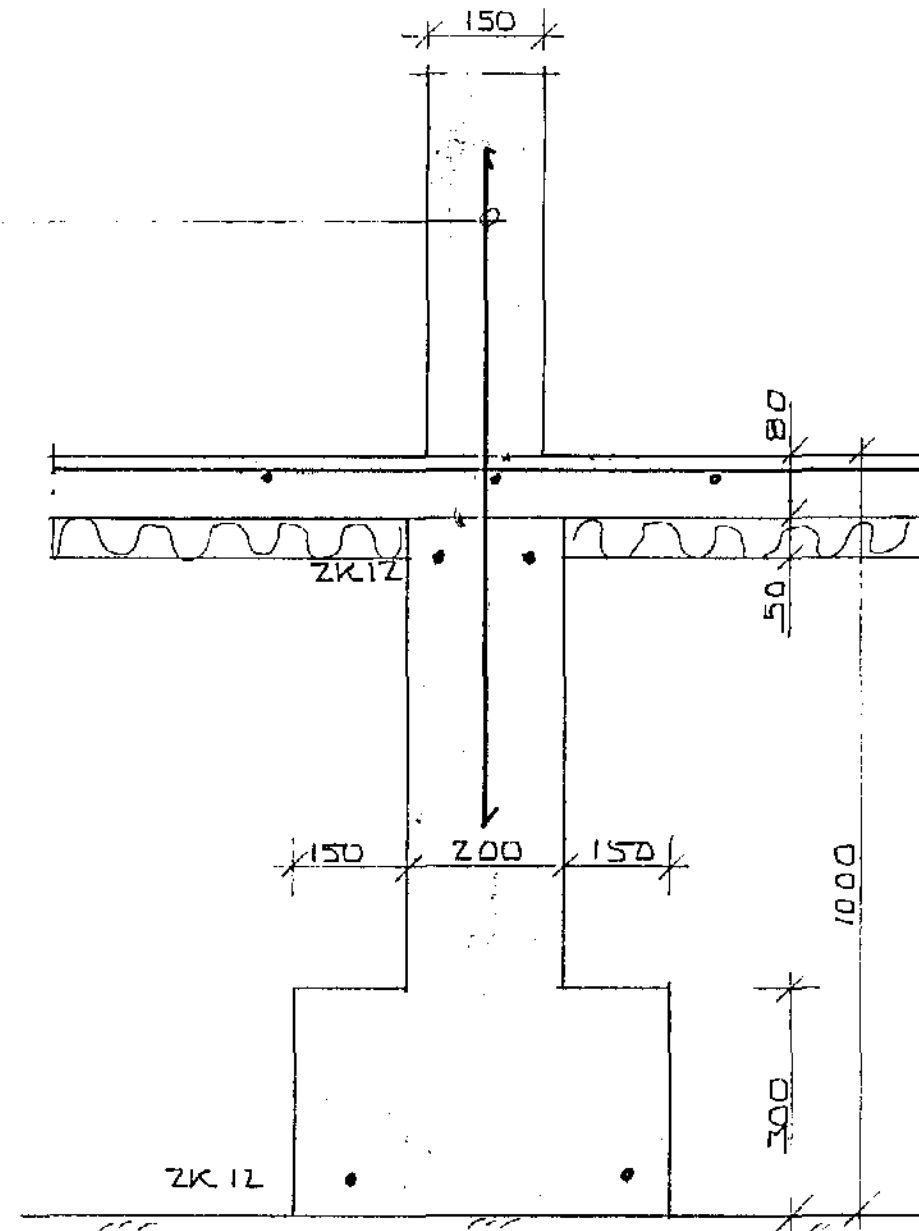
SNID F-F 1:10
