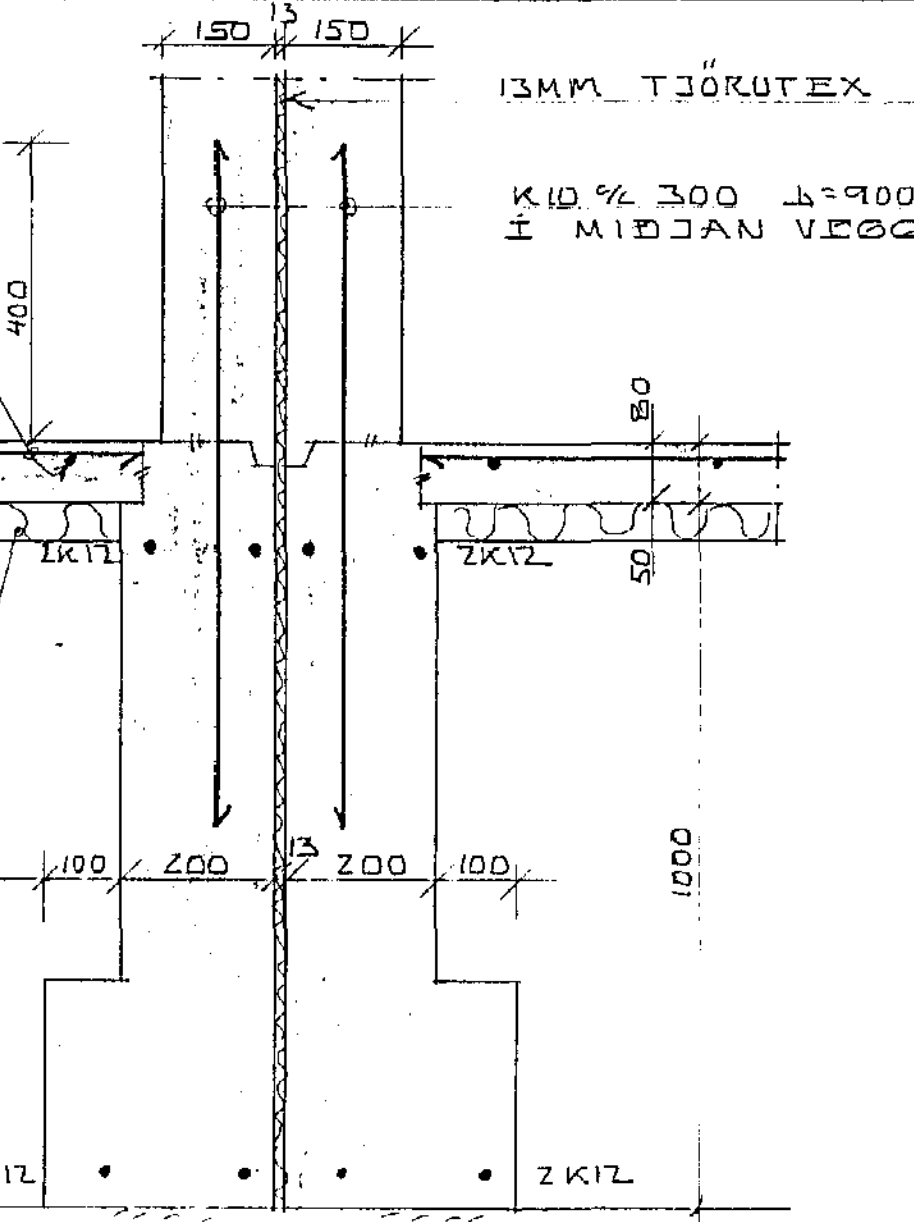
SNID C-C 1:10
