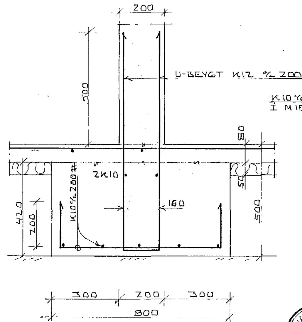
SNID C-C 1:10
