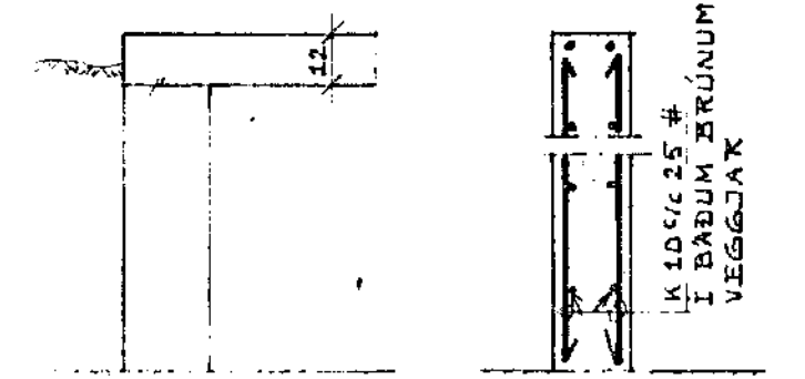
SNID F-F 1:20
