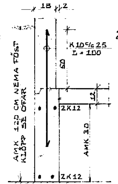
SNID E-E 1:20
