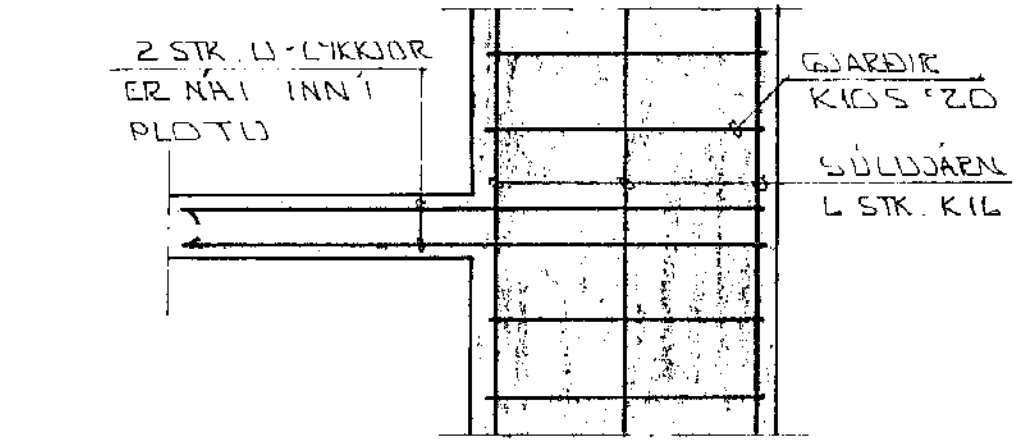
SNID X 1:20
