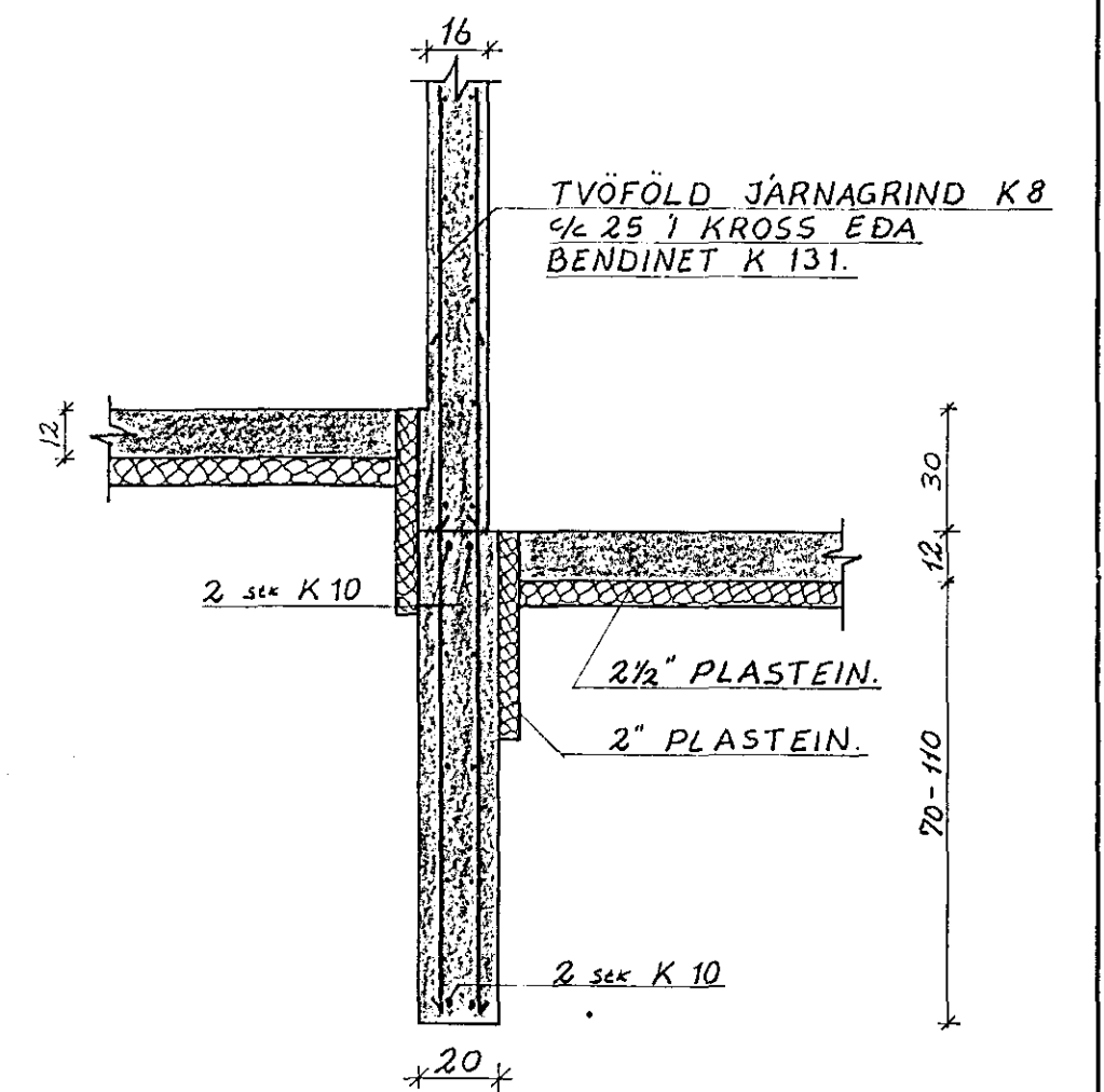
SNID C-C 1:20
