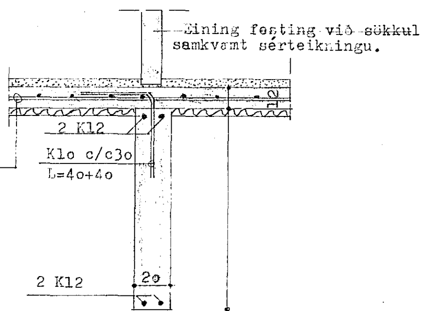
SNID B-B, M=1:20.
