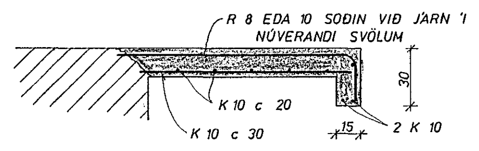
SNID D 1: 20
