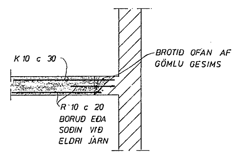
SNID A 1: 20
