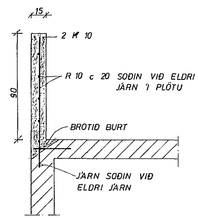
SNID B 1: 20
