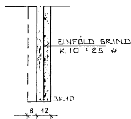
SNID A 1:20
