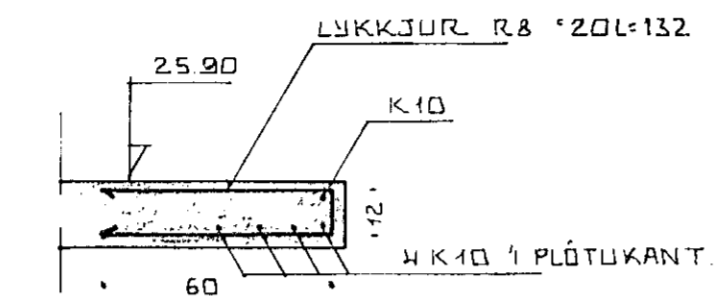
SNID C 1:20
