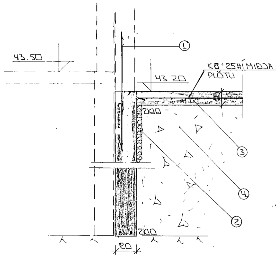
SNIB 2 1:20
