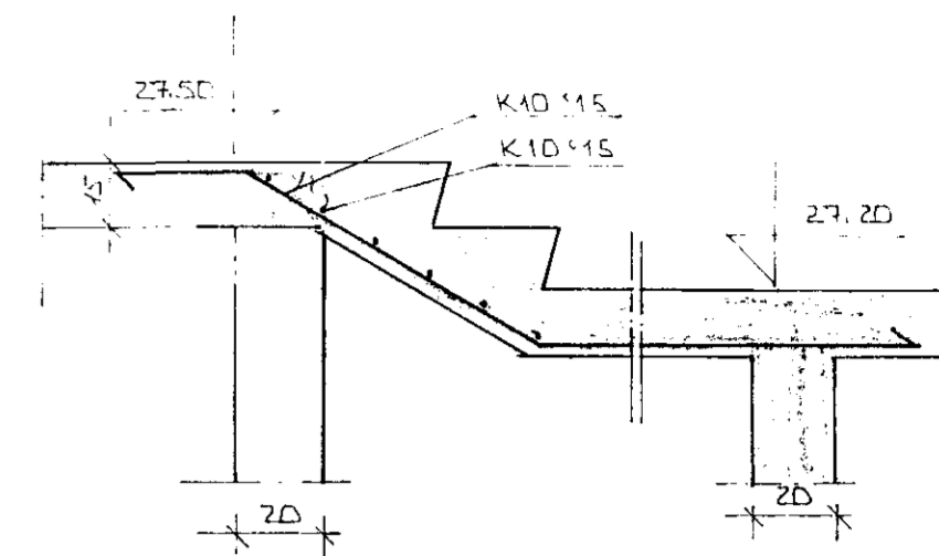
SNID A - A ~ 1:20
