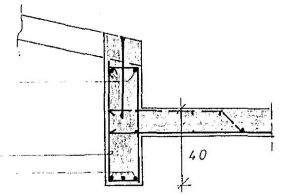
SNID H-H M 1:20
