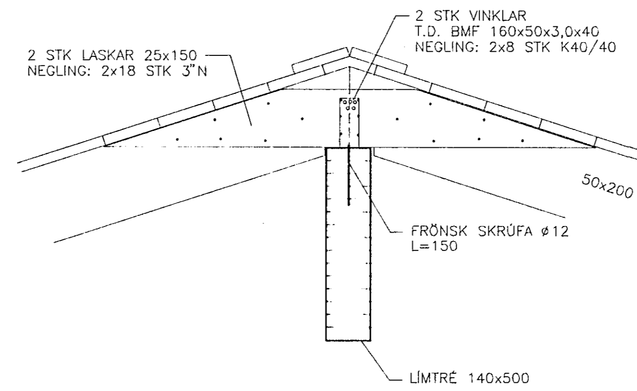
SNID C-C, 1:10
