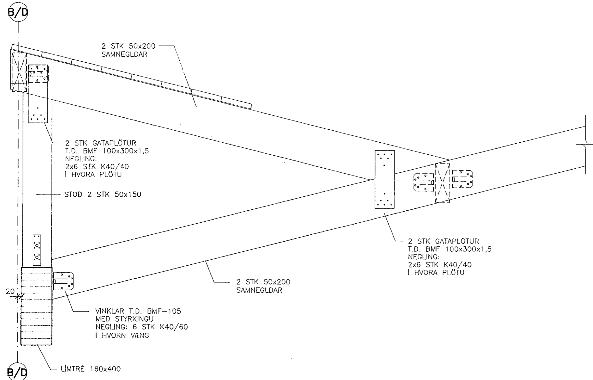
SNID E-E, 1:10
