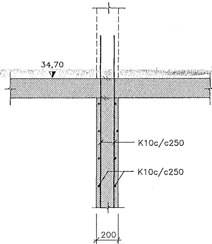
SNID E-E, 1:20
