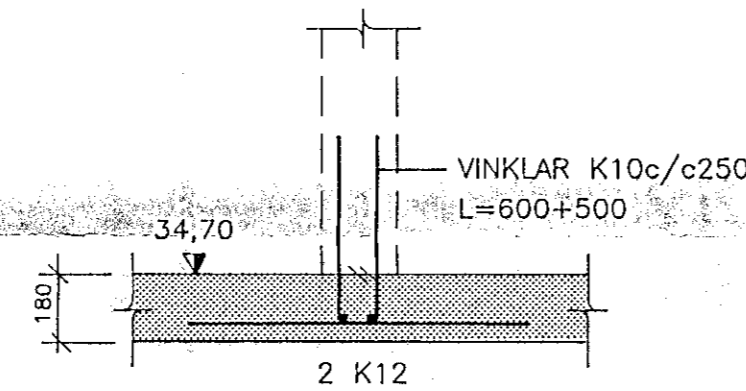
SNID F-F, 1:20
