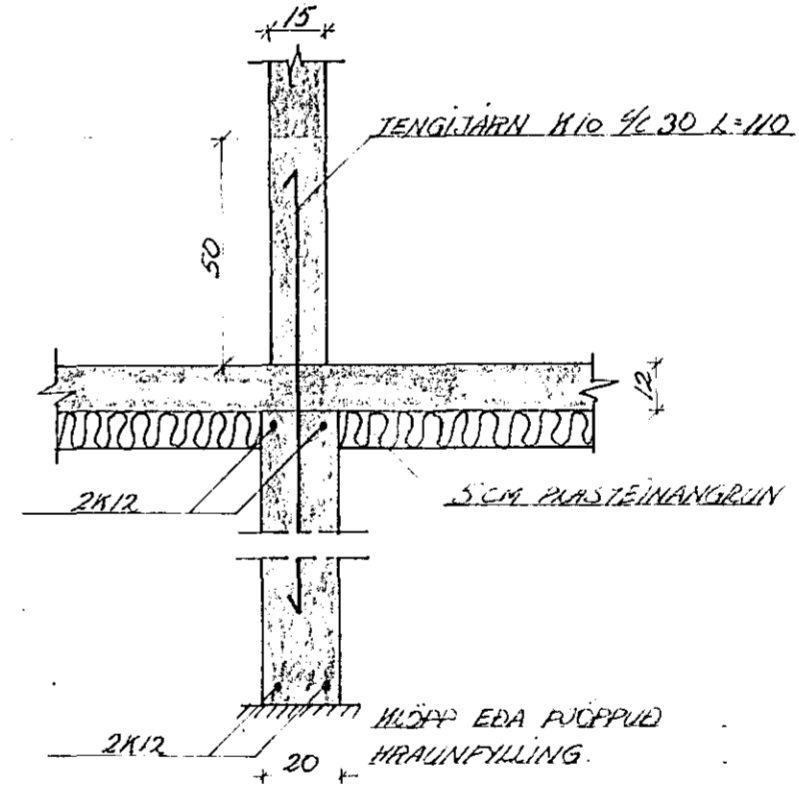
SNID C-C 1:20
