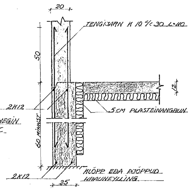
SNID C-C 1:20
