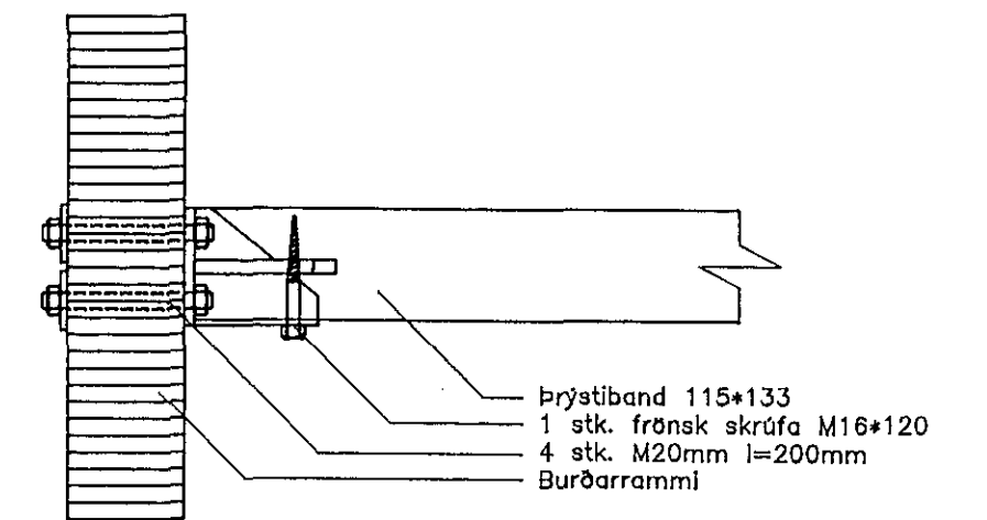
SNID B - B Mkv. 1:10
