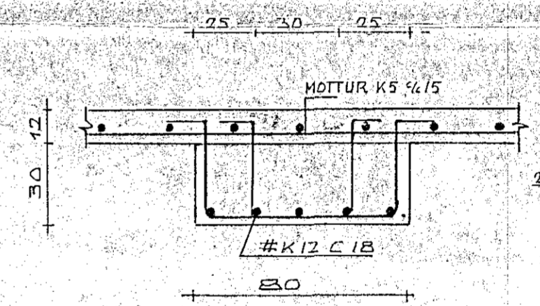
SNID C-C 1:20
