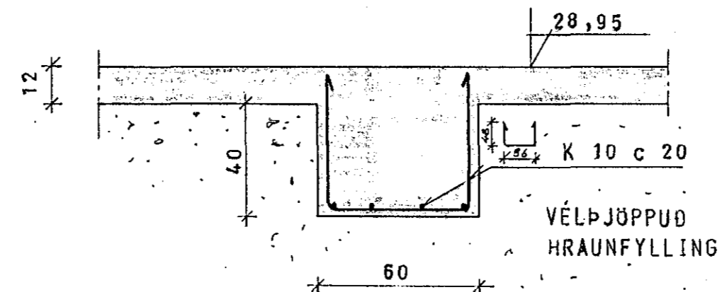
SNID C 1:20
