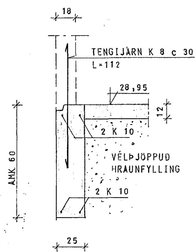
SNID A 1:20
