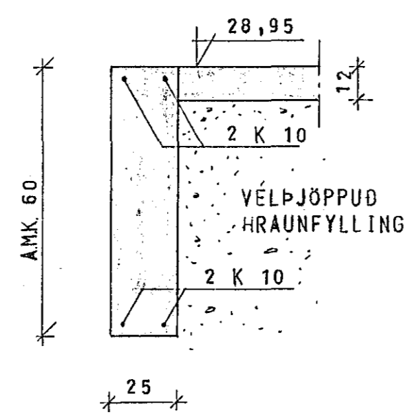
SNID B 1:20
