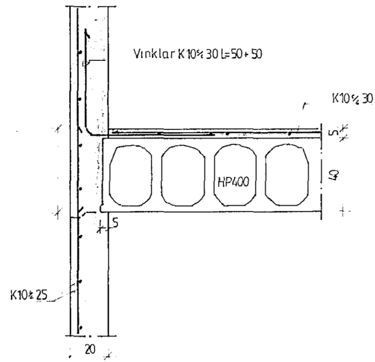
Snid C2 - C2 1:20
