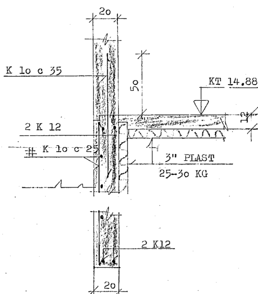
SNID E-E 1:20
