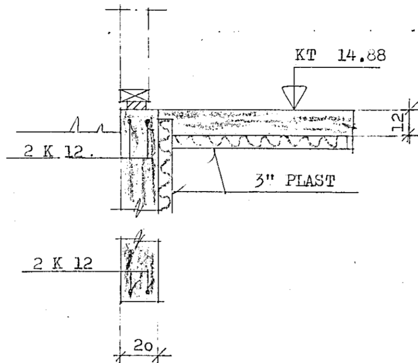
SNID E-E 1:20
