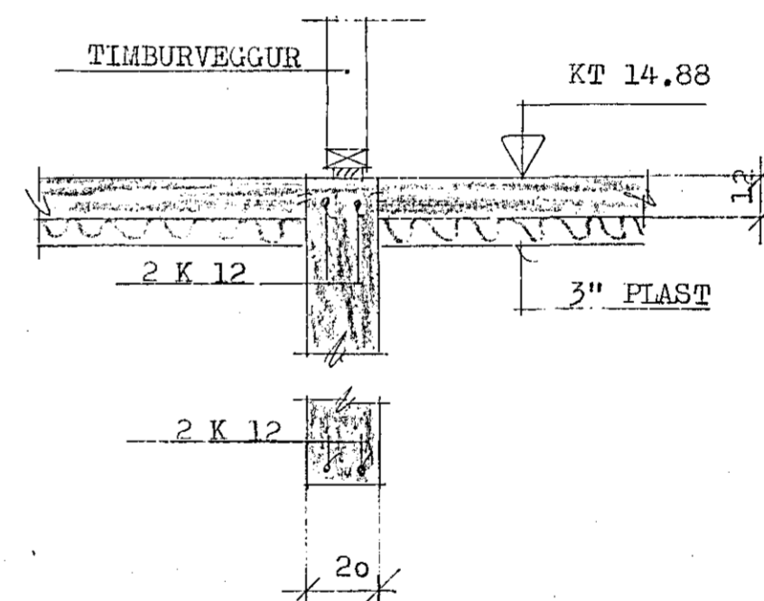
SNID F-F 1:20
