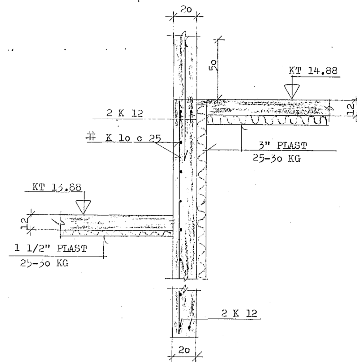
SNID F-F 1:20
