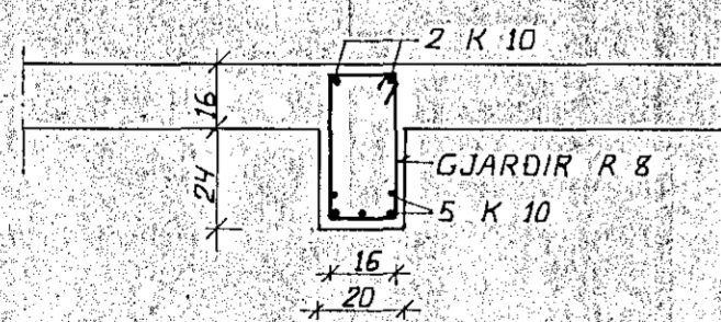
SNID B 1:20
