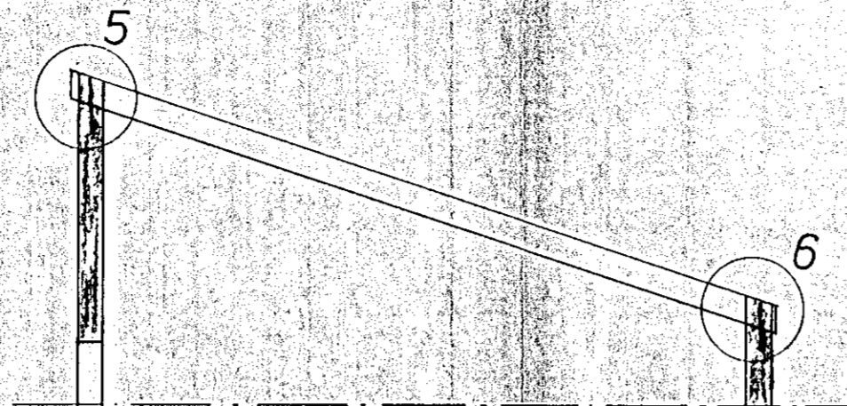
SNID C-C 1:50
