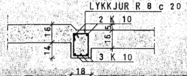
SNID B 1:20 IBITA B 01
