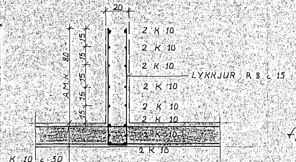
SNID A 1:20
