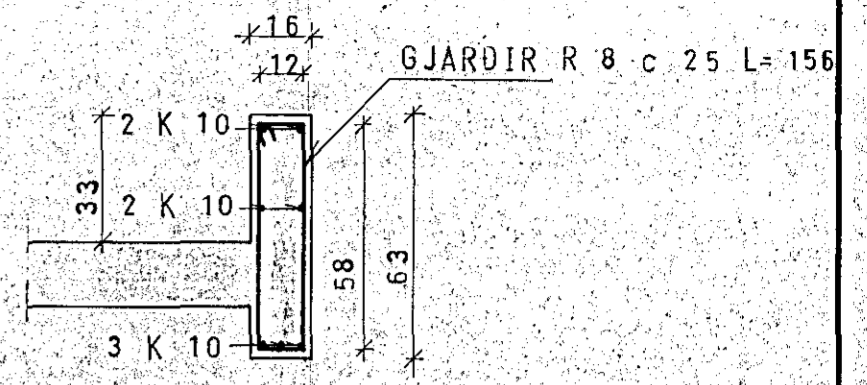
SNID A 1:20
