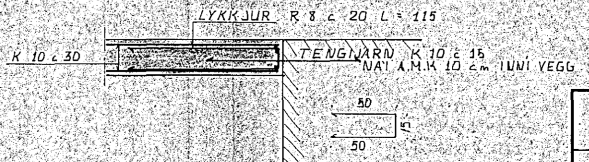
SNID B 1:20
