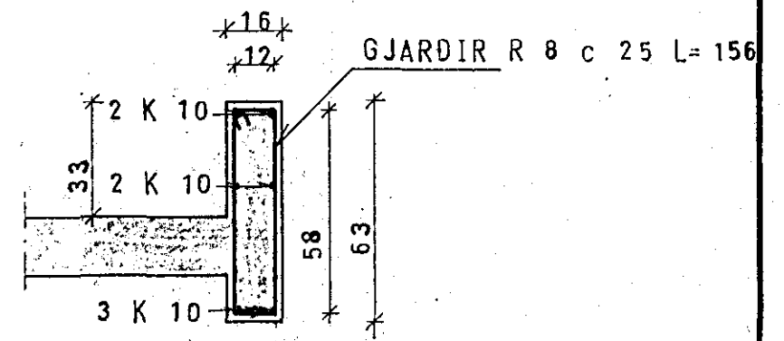
SNID A 1:20
