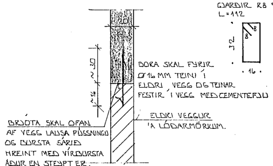
SNID B-B \approx 1:20
