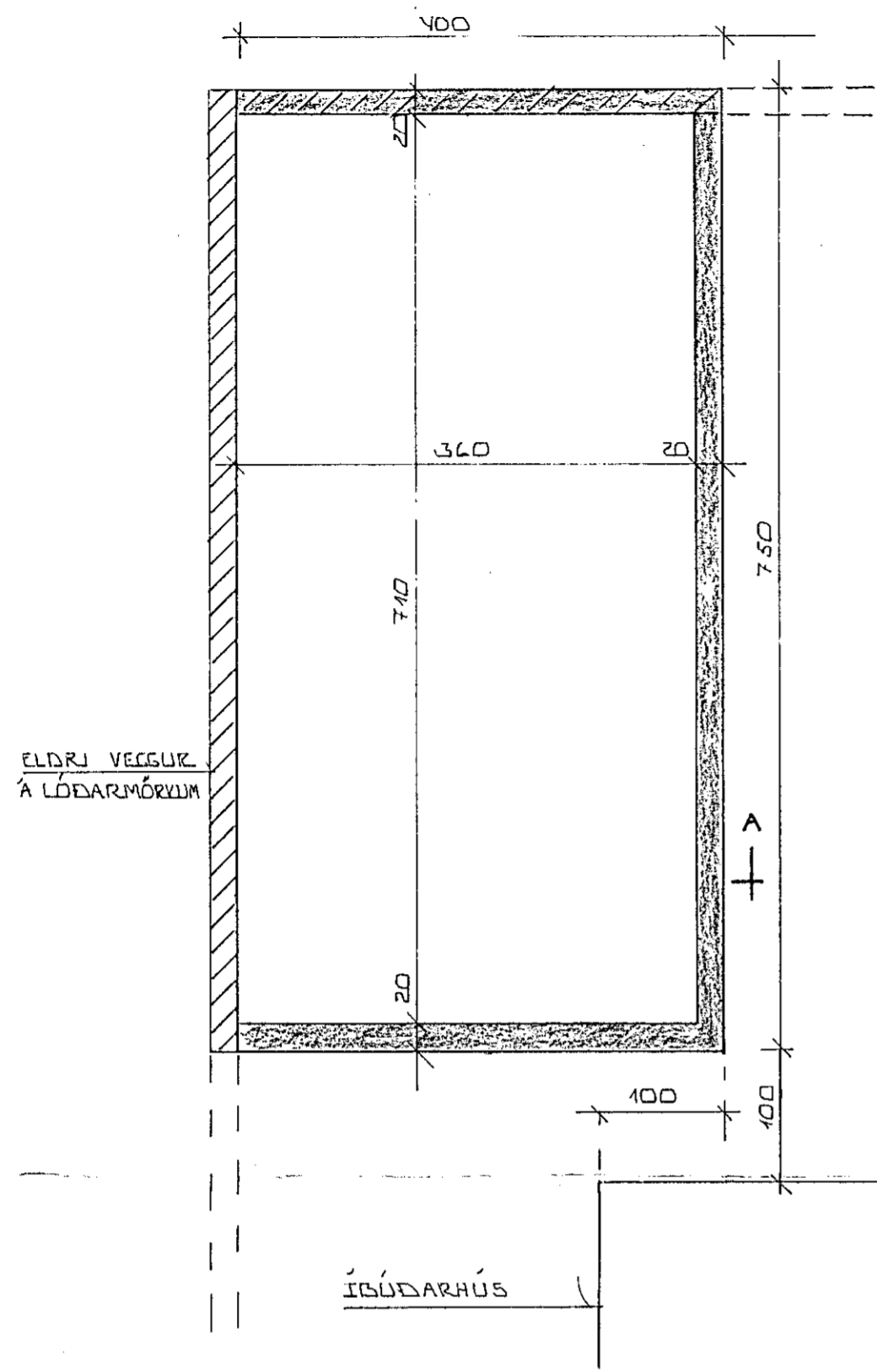
GRUNNMÝND UNDIRST. \approx 1:50
