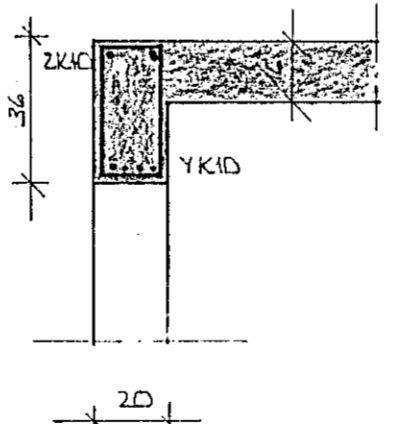
SNID C-C \approx 1:20
