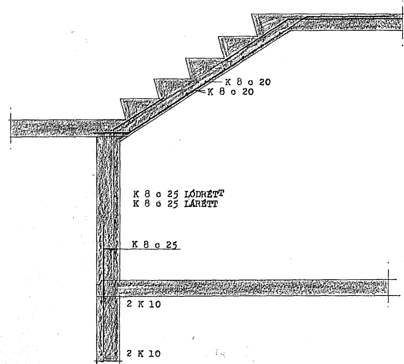
SNID - A 1:20 BL.1
