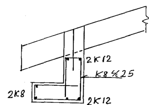
SNID C-C 1:20
