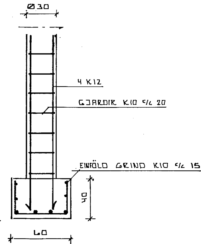
SNID S1 1:20
