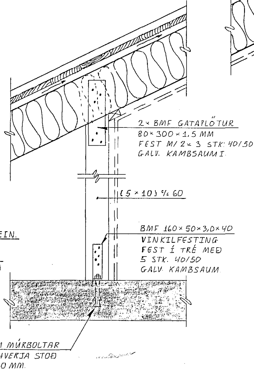
SNID B 12 -B 12 . 1:10
