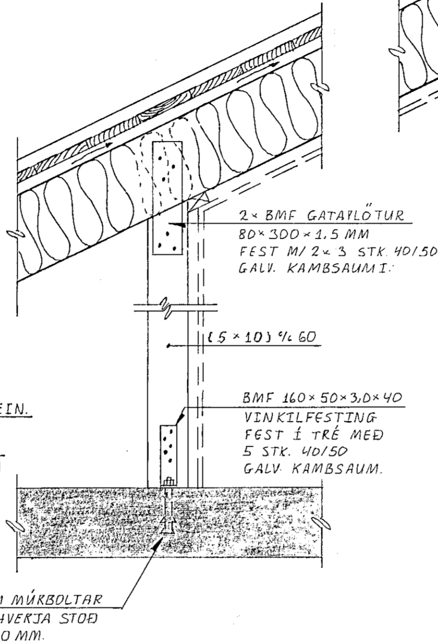
SNID B 12 -B 12 . 1:10
