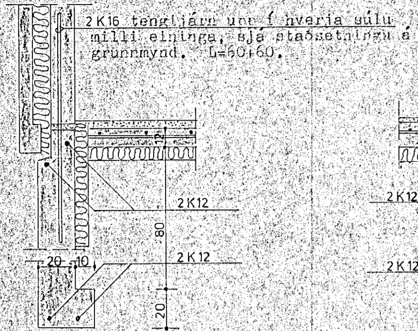
SNIP A-A, M=1:20.
