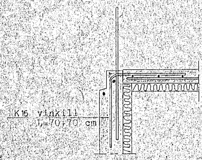
SNIP D-D, M=1:20.
