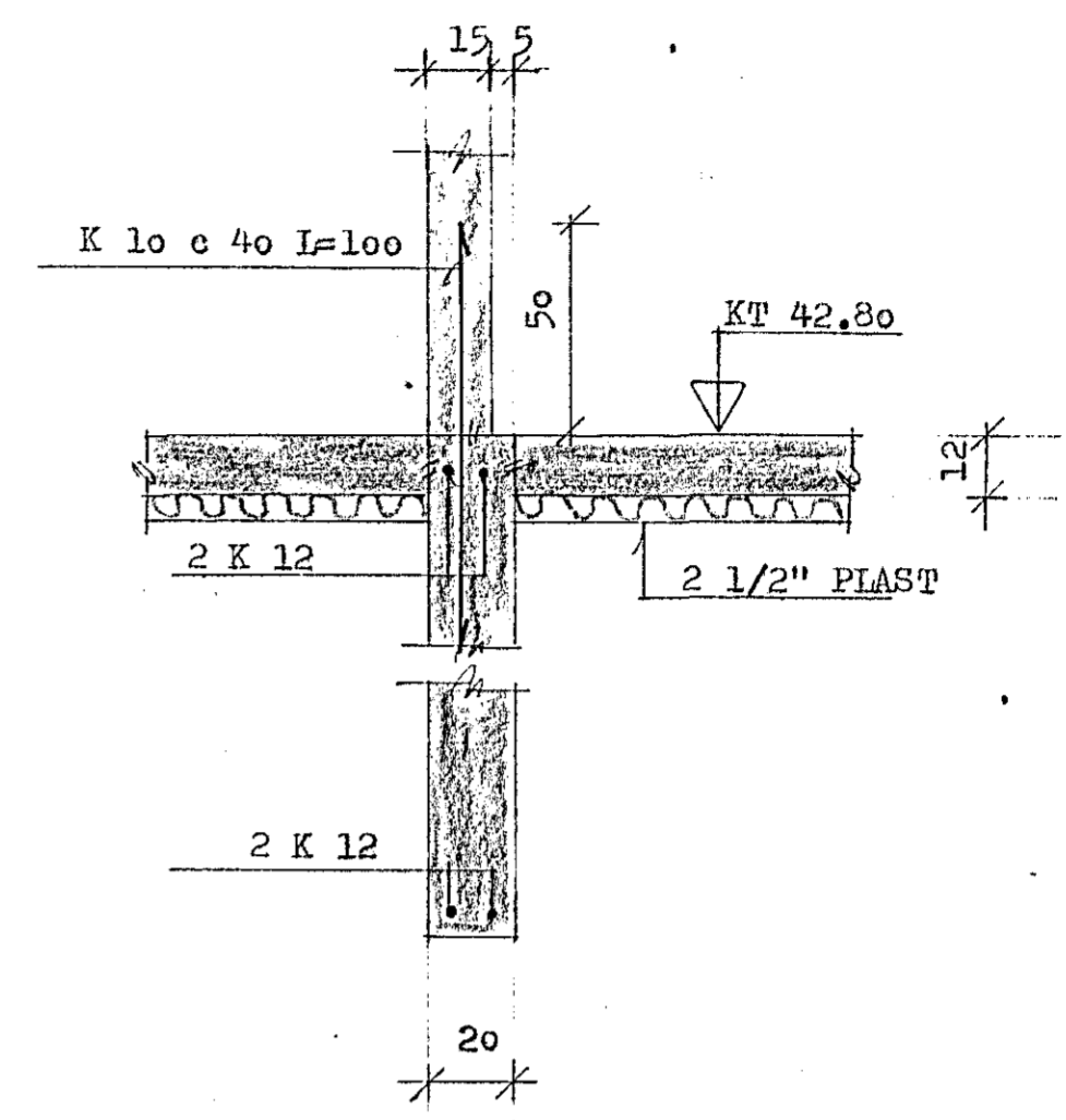
SNID C-C 1:20
