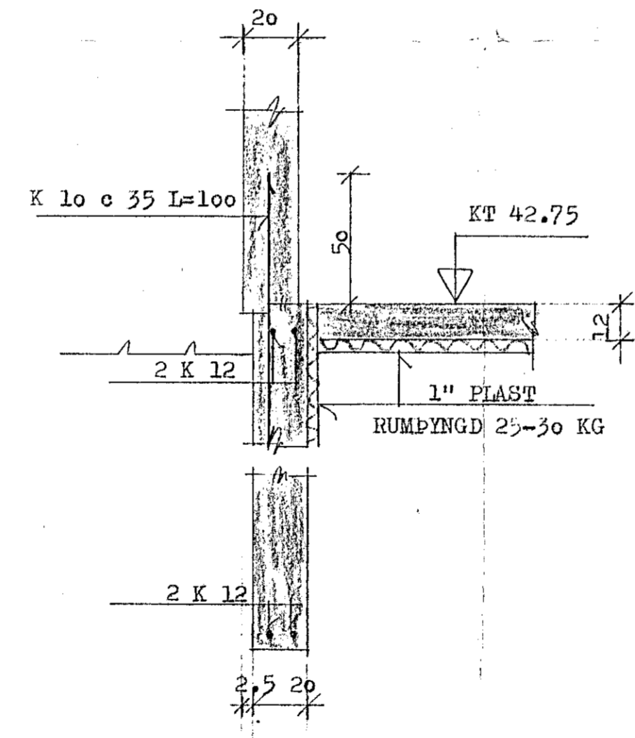
SNID E-E 1:20
