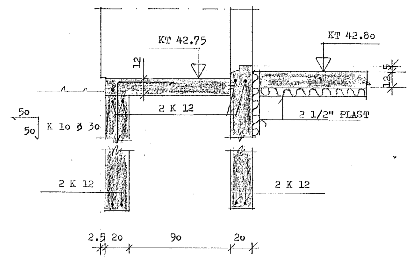
SNID E-E 1:20
