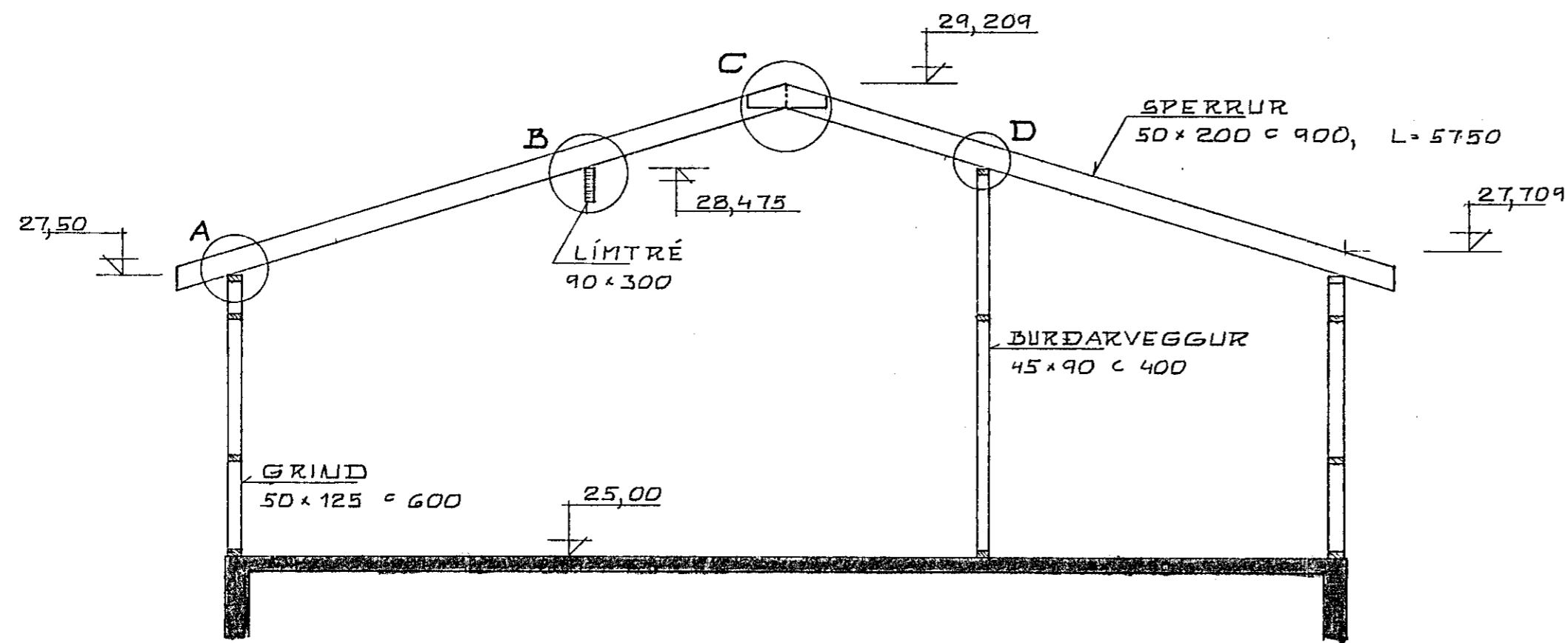
SNID 1-1 1:50
