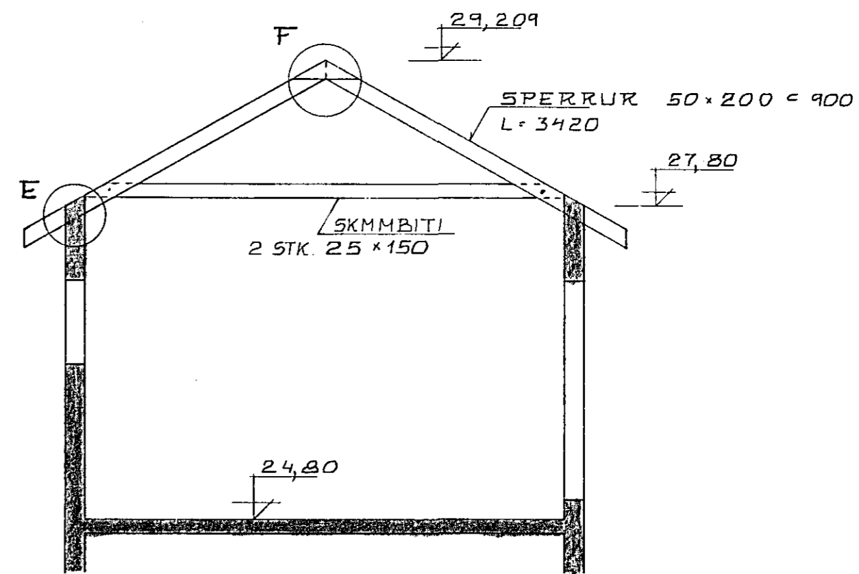
SNID 2-2 1:50
