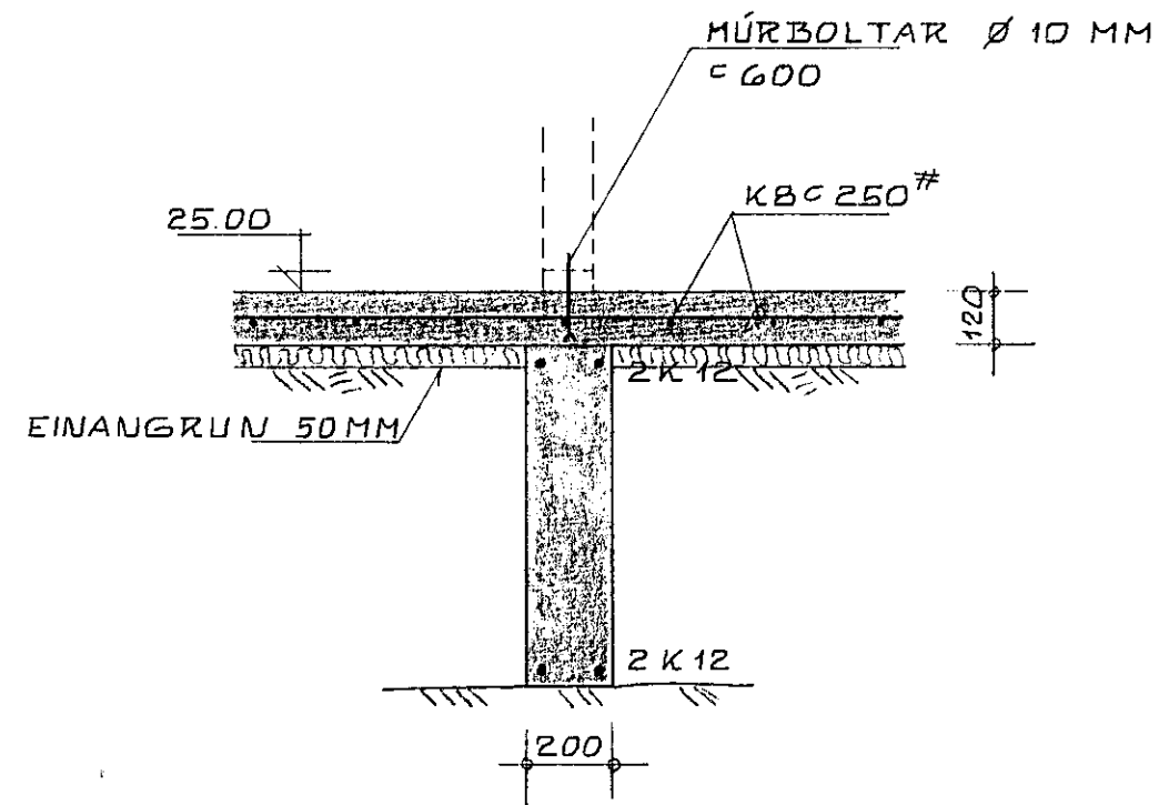
SNID 3-3 1:20
