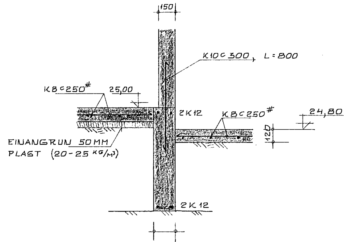
SNID 4-4 1:20
