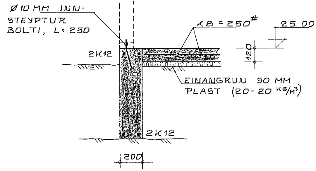
SNID 2-2 1:20
