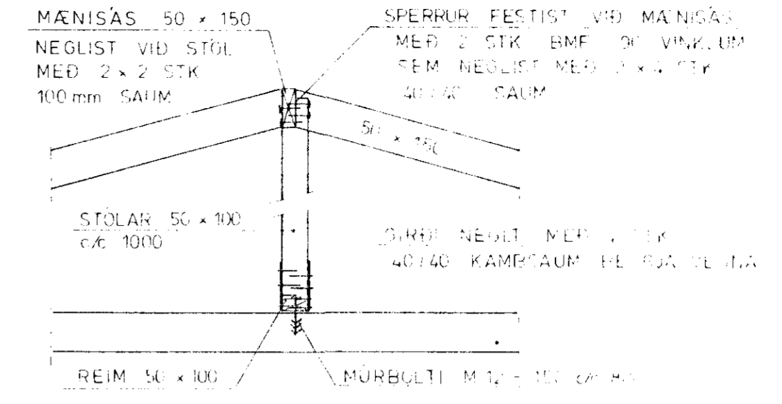
SNID A 1:20
