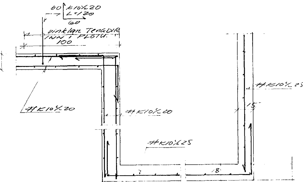
SNID X-X 1:20
