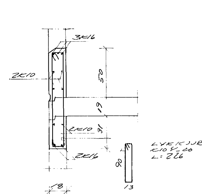
SNID Y-Y 1:20
