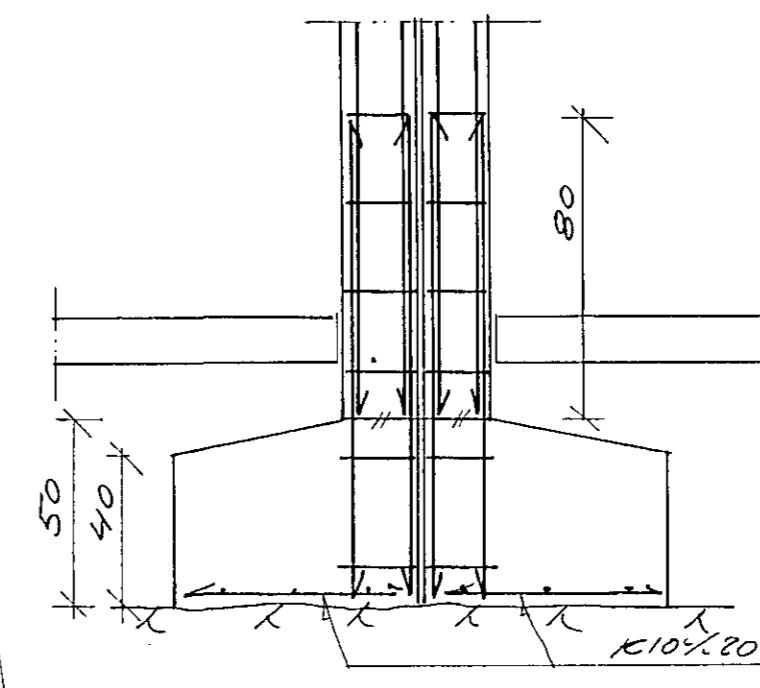
SNID c-c 1:20
