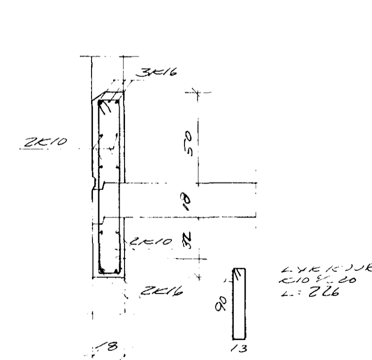
SNID Y-Y 1:20
