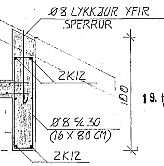
SNID K-K
