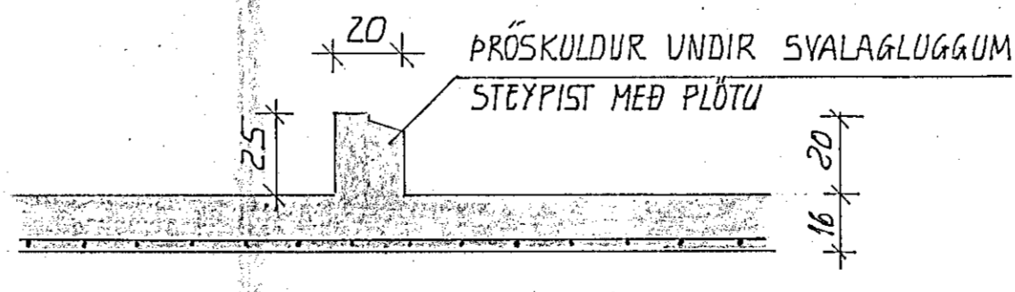
SNID M-M
