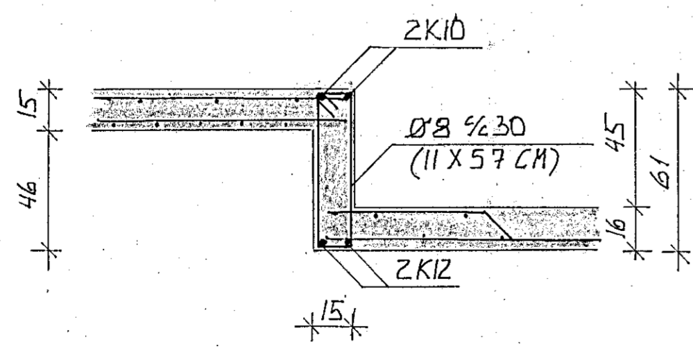
SNID L-L
