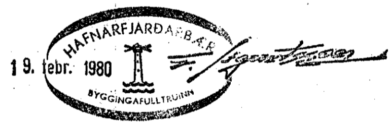
SNID K-K
