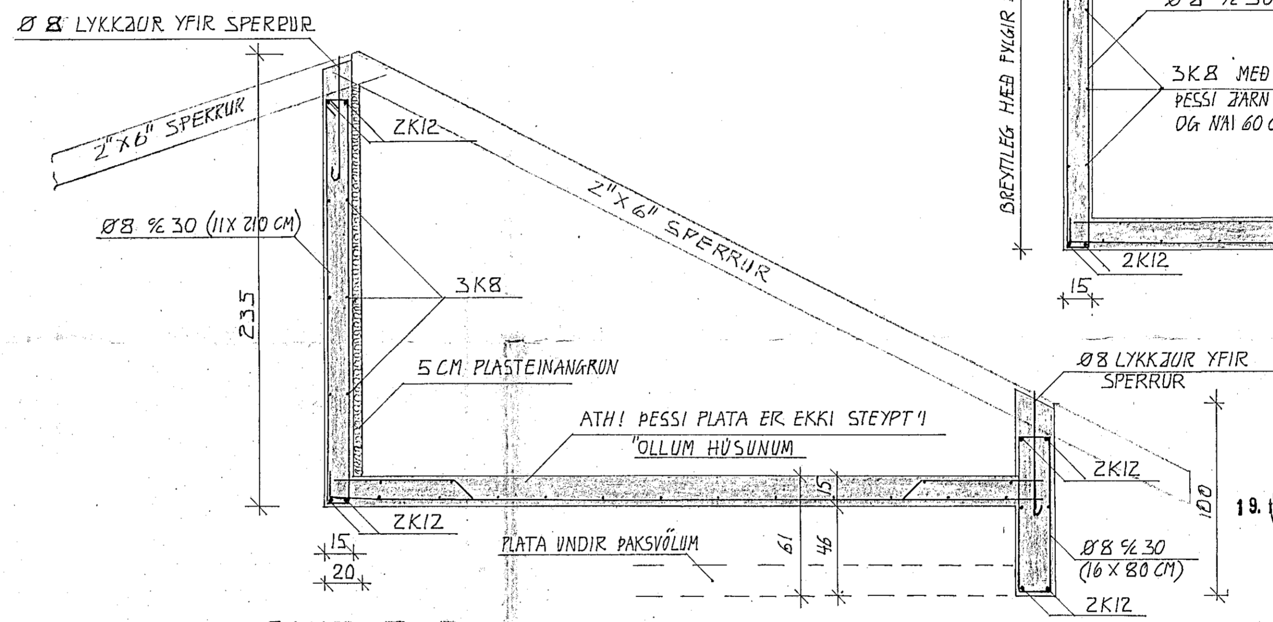
SNID K-K
