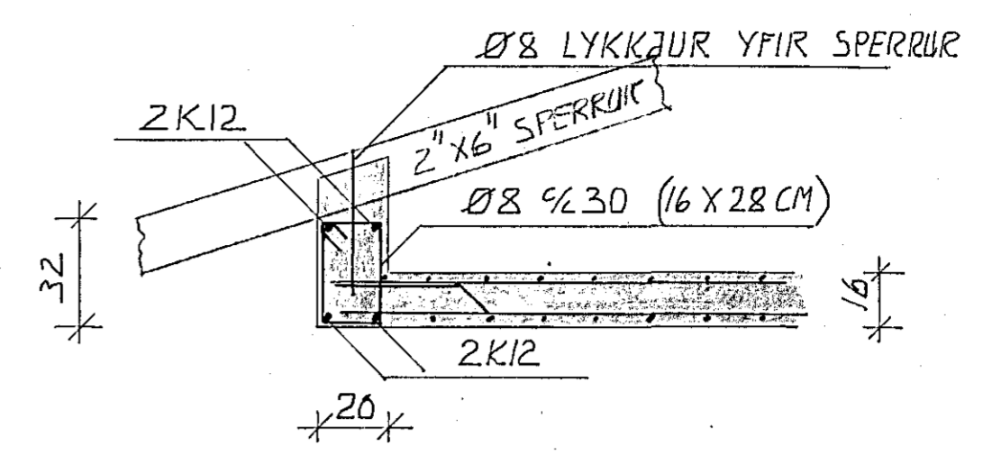
SNID H-H
