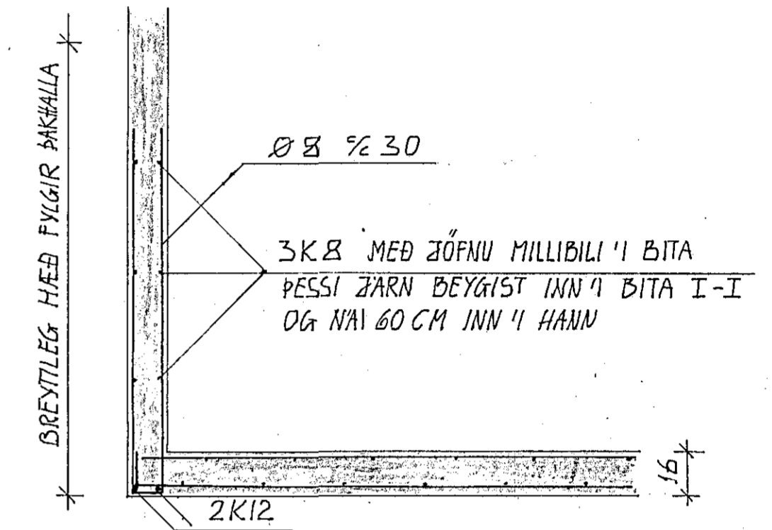
SNID N-N
