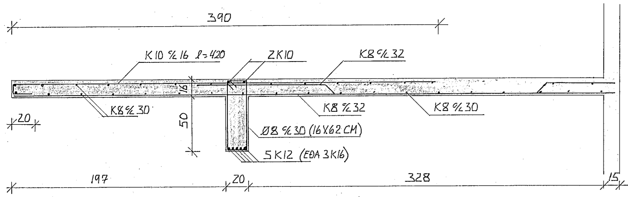
SNID G-G
