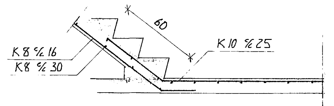
SNID 2-2
