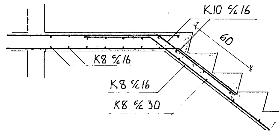
SNID 1-1
