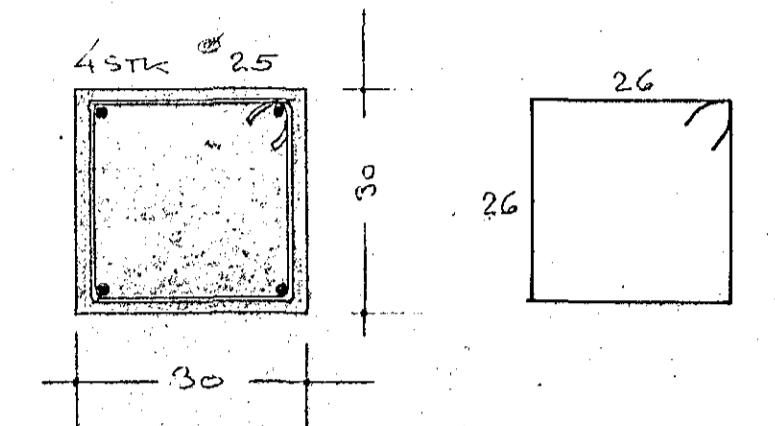
SNID M-M 1:10
