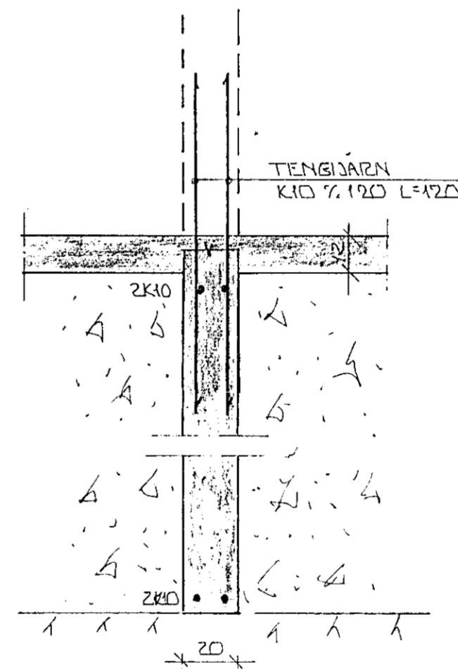
SNID 3 ~1:20
