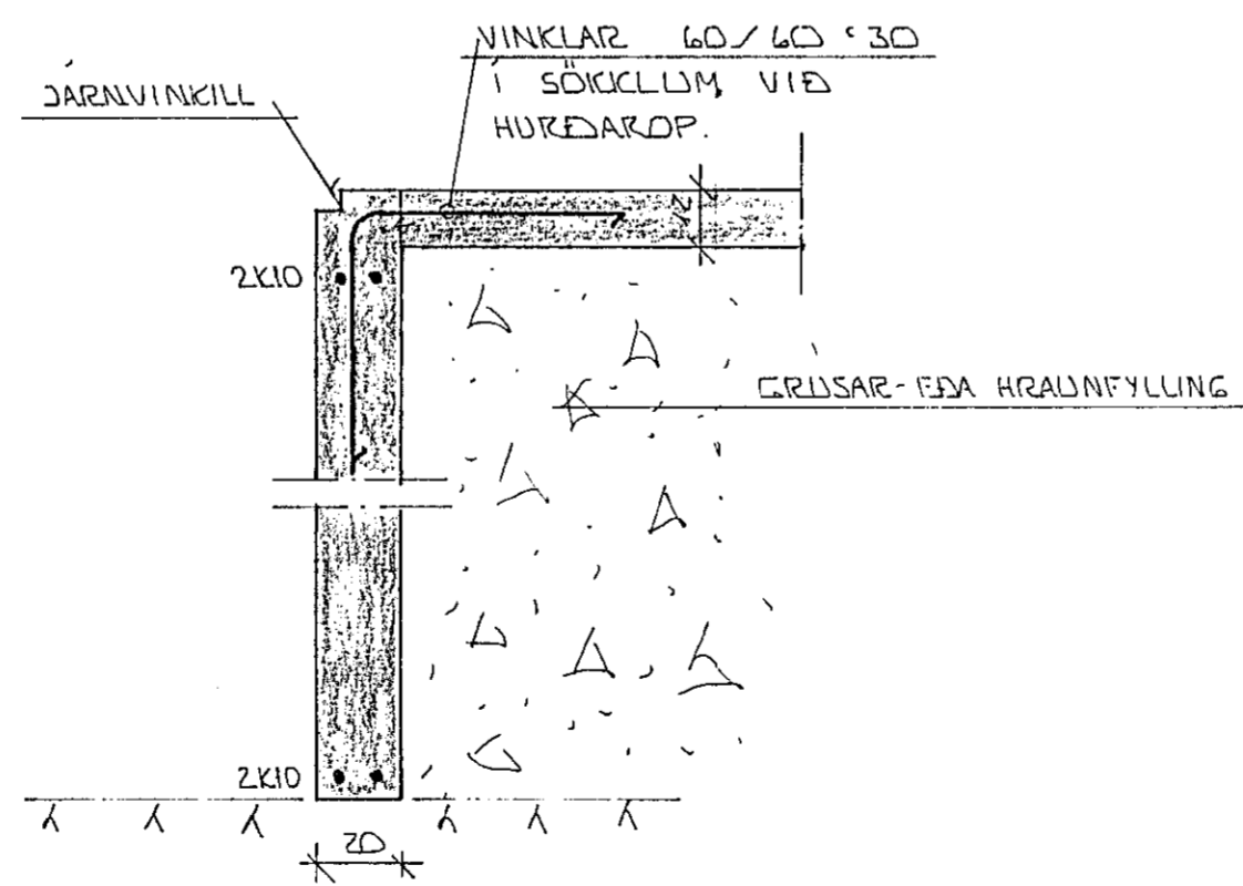
SNID 2 ~1:20
