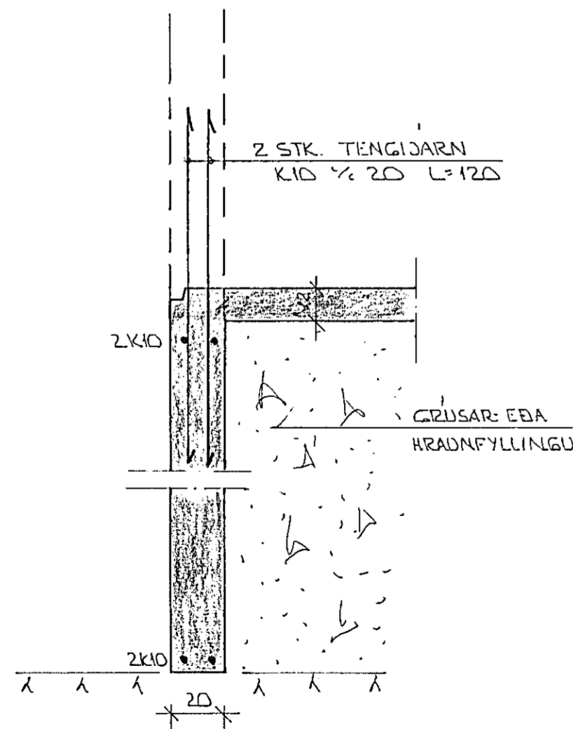
SNID 1 ~1:20
