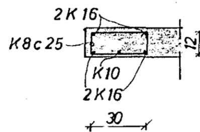
SNID C 1:20
