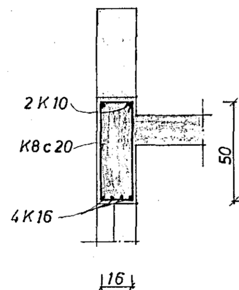
SNID B 1:20
