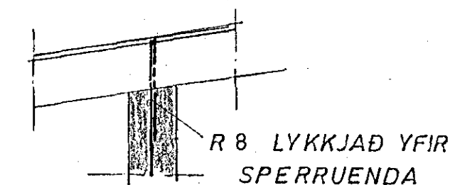
SNID B 1:20
