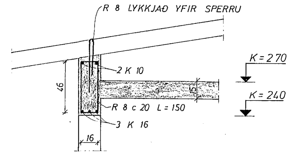
SNID A 1:20
