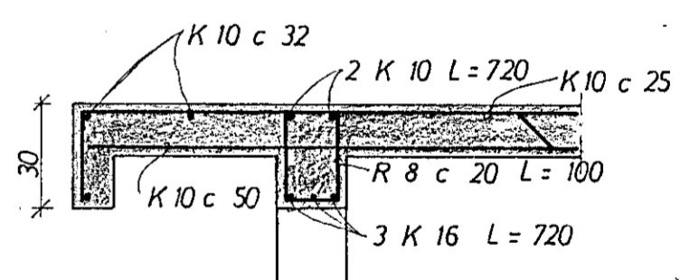
SNID B 1:20
