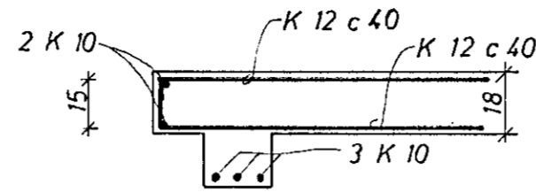
SNID B 1:20
