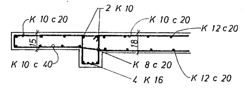
SNID A 1:20
