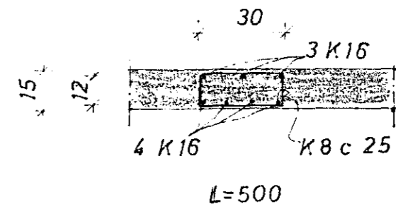
SNID C 1:20
