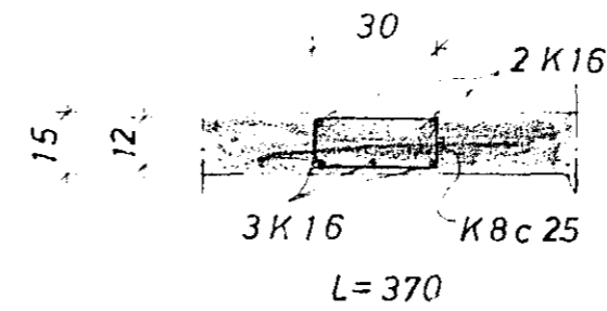
SNID A 1:20
