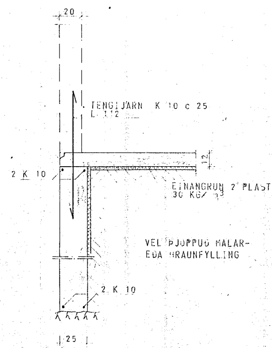
SNID B 1:20
