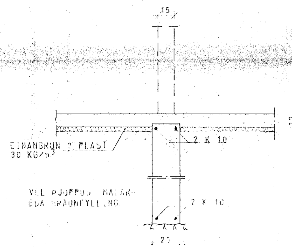
SNID F 1:20
