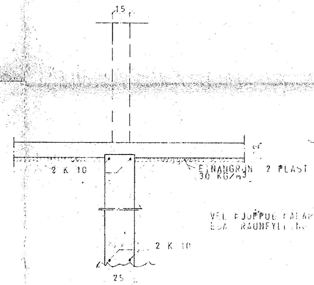
SNID H 1:20
