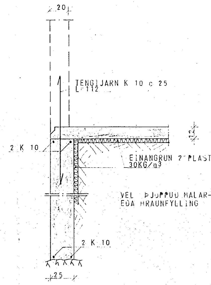
SNID A 1:20
