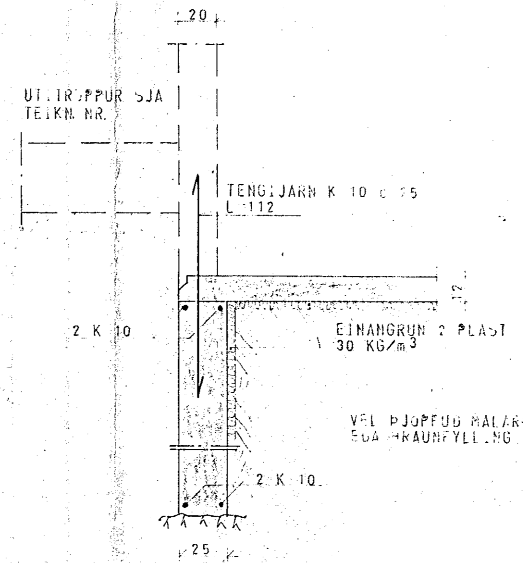
SNID C 1:20
