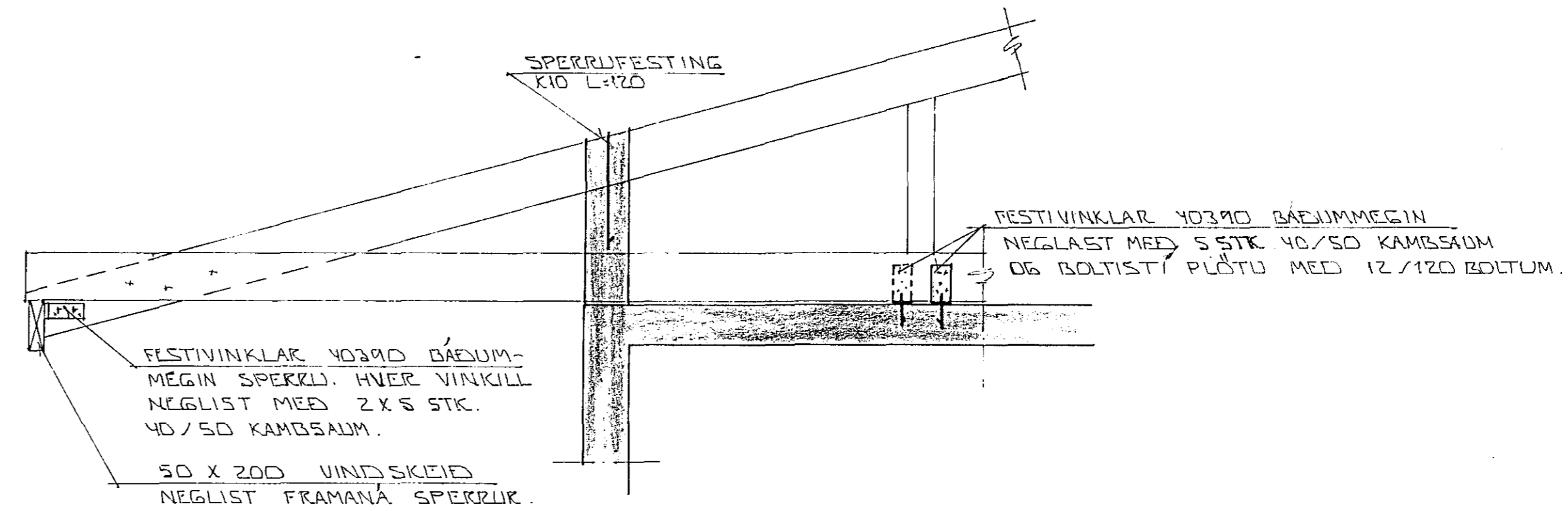
SNID 7-7 - 1:20
