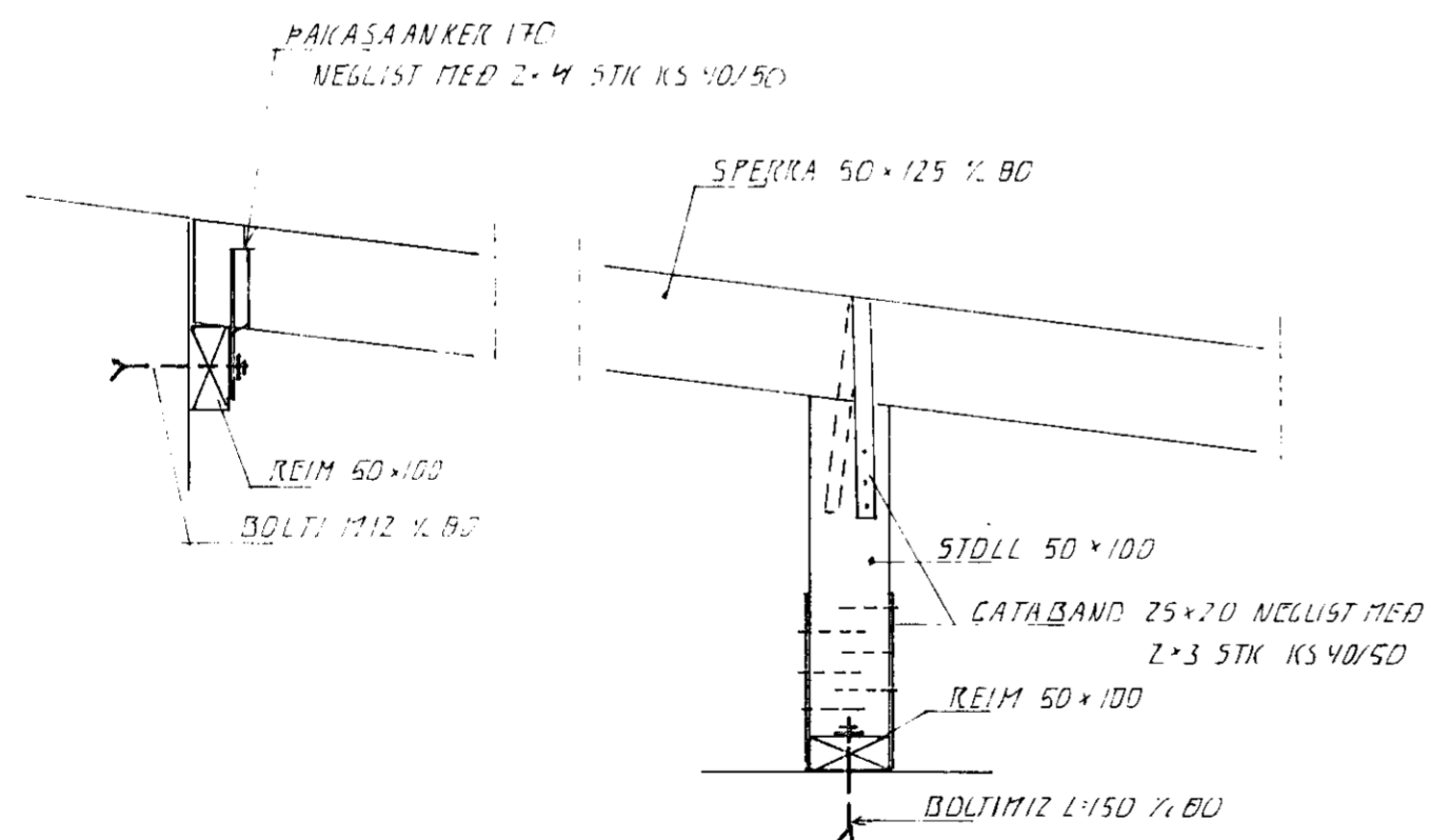
SNIB 1-1, 1:10
