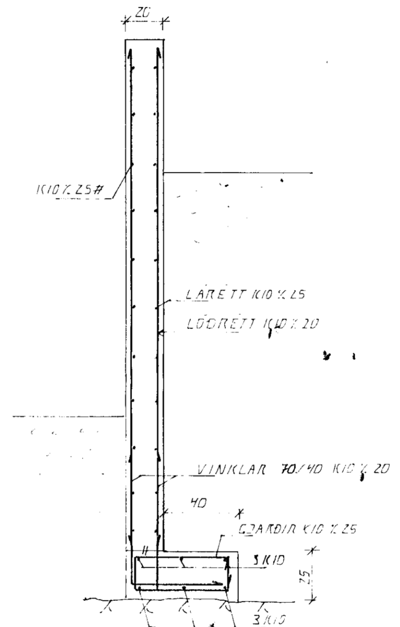
SNIB 2, 1:20
