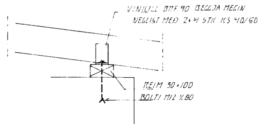
SNIB 2, 1:20
