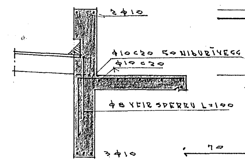
SNIB - C 1:20
